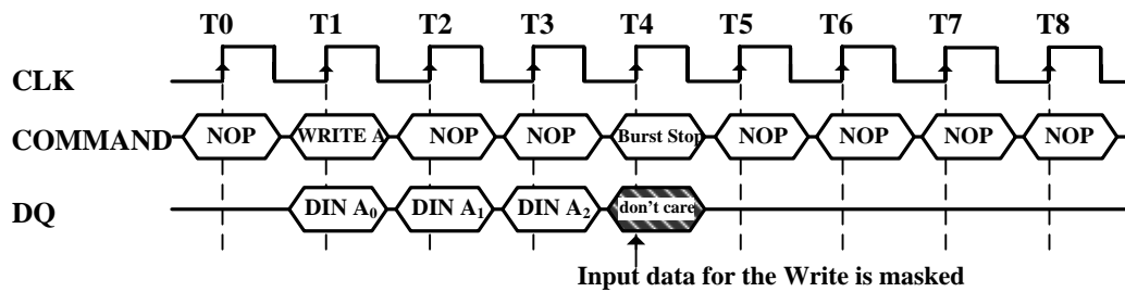
Figure 17. Termination of a Burst Write Operation (Burst Length = X)
