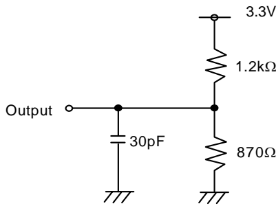
Figure 18.1 LVTTTL D.C. Test Load (A)
