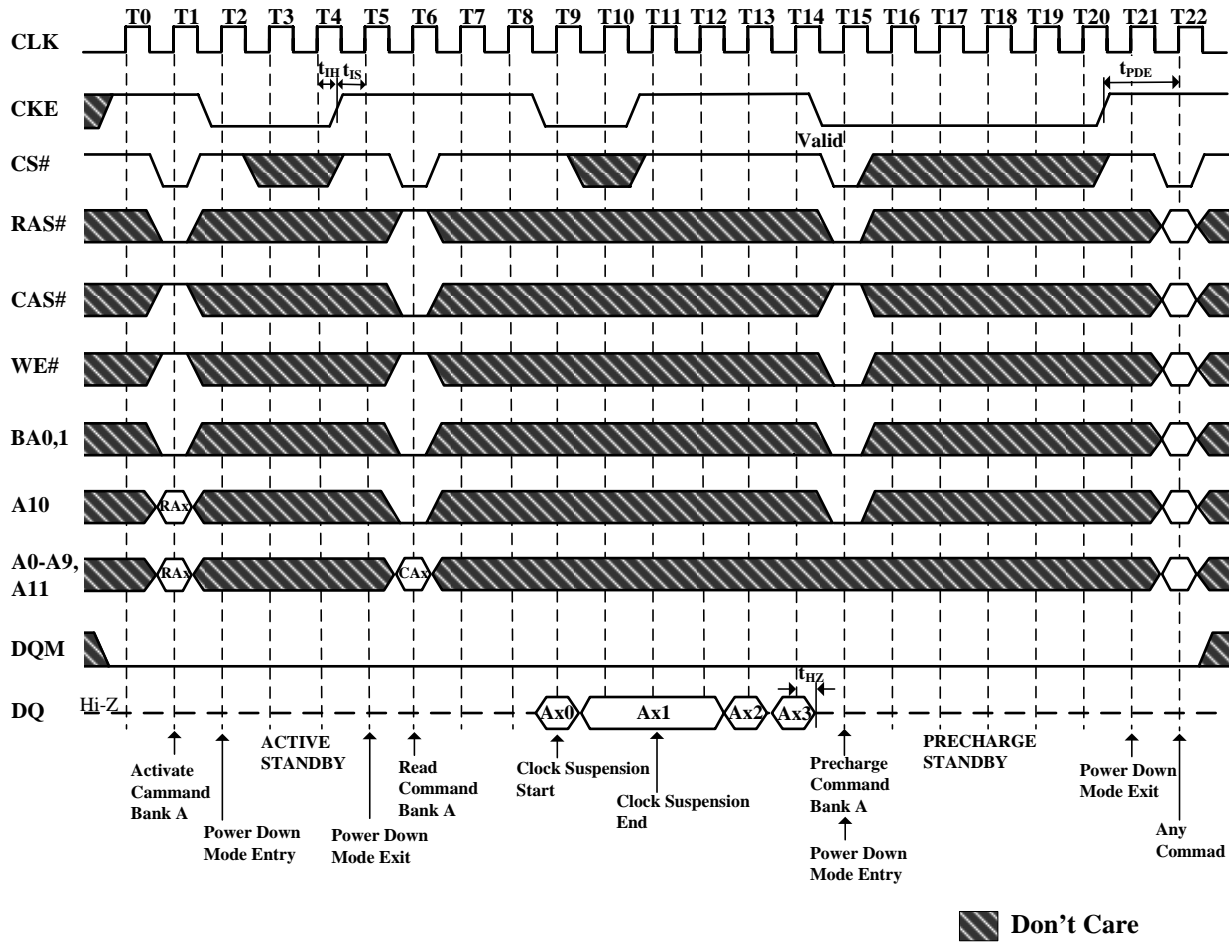
Figure 26. Power Down Mode and Clock Suspension (Burst Length=4, CAS# Latency=3)
