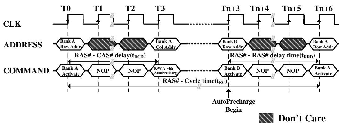
Figure 3. BankActivate Command Cycle (Burst Length = n, CAS# Latency = 3)
