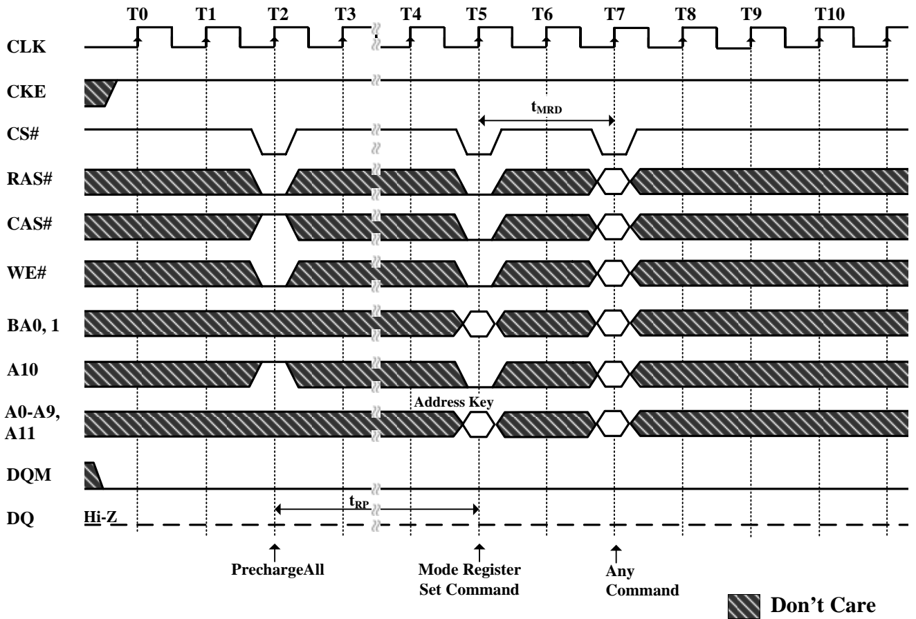
Figure 15. Mode Register Set Cycle
