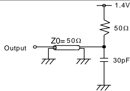
Figure 18.2 LVTTTL A.C. Test Load (B)
