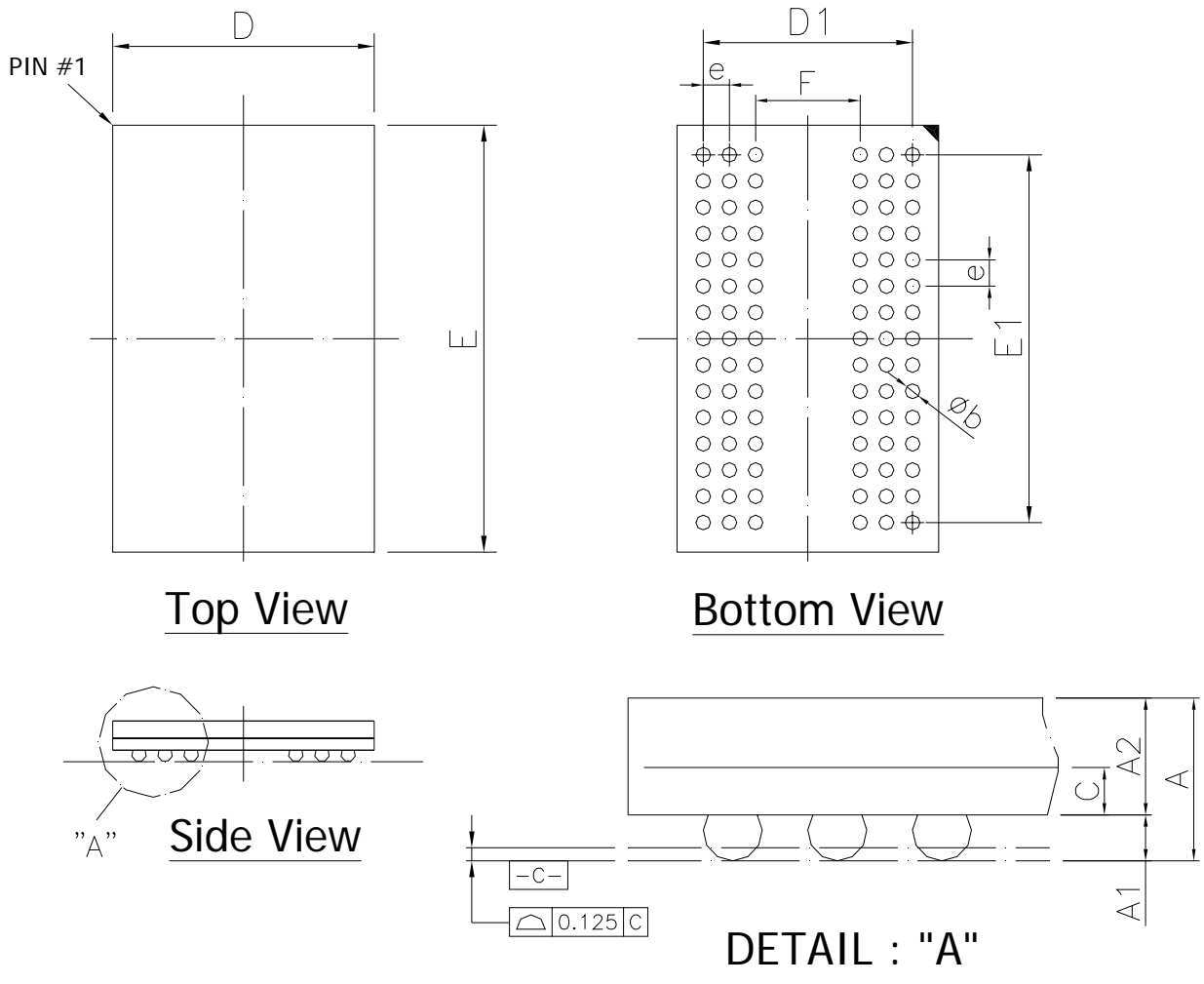
Figure 43. 90 ball (8mm x 13mmx1.4 mm) LFBGA Package Outline Drawing Information
